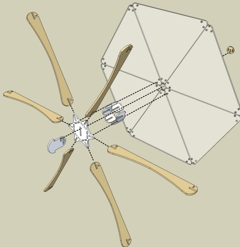
Exploded Parts
