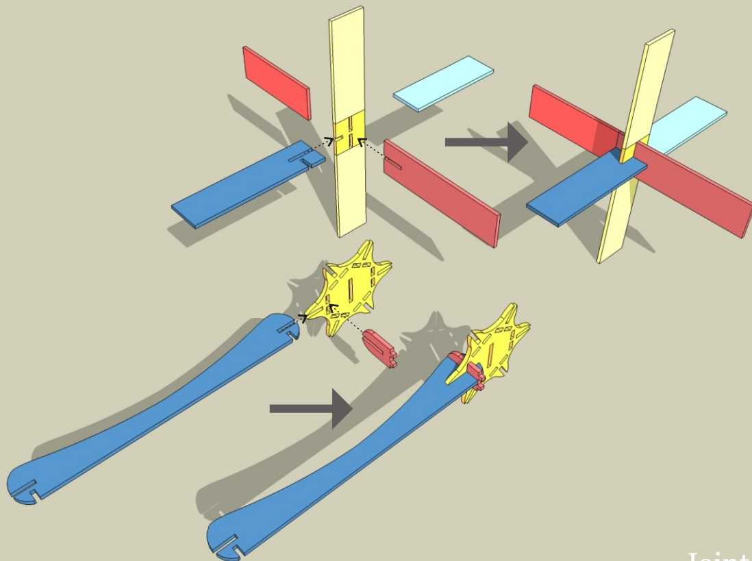
Joint Principles
