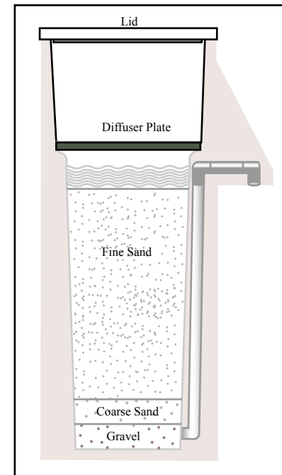
Figure by MIT OpenCourseWare. Diagram of Biosand Filter
