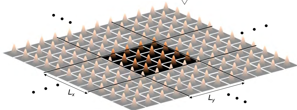
Fig. 6.26. An example of a 2-d periodic material.
