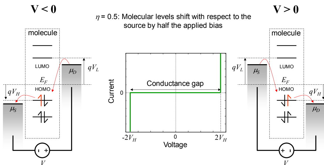
Fig. 3.16. When \eta = 0.5 , conduction always occurs through the molecular orbital closet to the Fermi Energy. In this example that is the HOMO, irrespective of the polarity of the applied bias. Adapted from F. Zahid, M. Paulsson, and S. Datta, „Electrical conduction in molecules“. In Advanced Semiconductors and Organic Nanotechniques , ed. H. Korkoc. Academic Press (2003).
