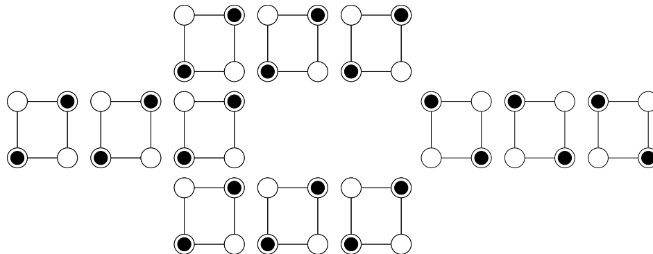
Fig. 7.21. A cellular automata inverter.
