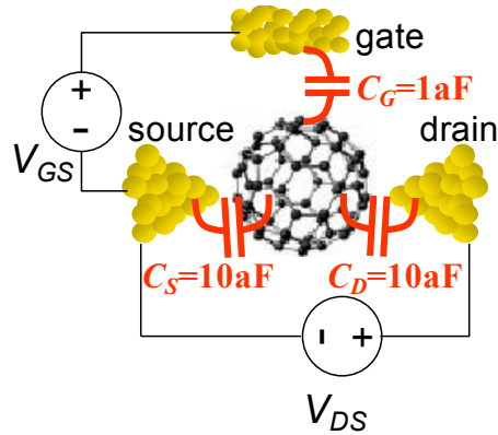
Fig. 5.33. The geometry of a C60 FET. In addition take the temperature to be T = 1\text{K} , and the molecular energy level broadening, \Gamma = 0.1\text{eV} . The LUMO is at -4.7\text{eV} and the Fermi Energy at equilibrium is E_F = -5.0\text{eV}
