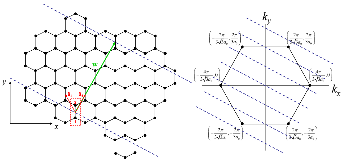
For a (0,4) tube \mathbf{w} = 2\sqrt{3}a_0\hat{x} + 6a_0\hat{y} . Thus, the allowed values of \mathbf{k}_\perp are given by Fig. 6.35. At left, a (0,4) zigzag nanotube. At right, the K points of graphene.
