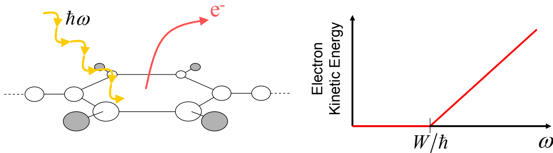
Fig. 1.16. The photoelectric effect: above a critical frequency, light can liberate electrons from a solid.
