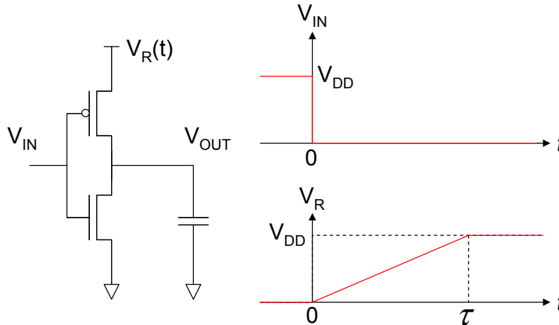
Fig. 7.18. An adiabatically-driven inverter.
