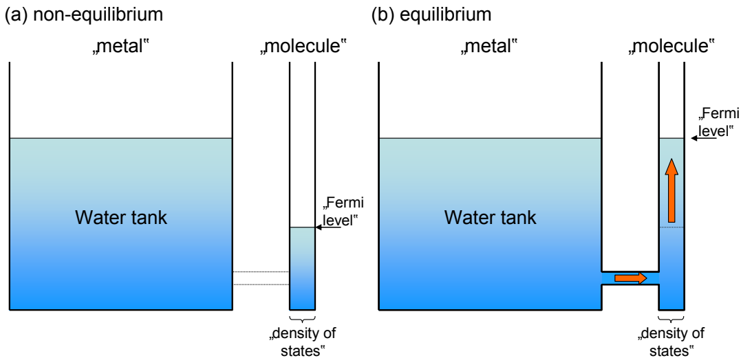
Fig. 3.5. An analogy for electron transfer at the interface between a metal and a molecule. The size of the water tank is equivalent to the density of states. The Fermi level is equivalent to the water level. If the „metal“ has a sufficiently large density of states, then the change in its water level is imperceptible.
