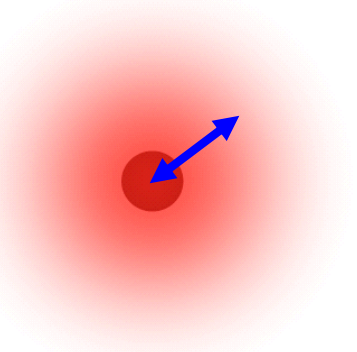
Fig. 6.8. The interaction between a nucleus and its frontier atomic orbital is known as the self energy.
