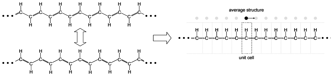
Fig. 6.18. The simplest model for polyacetylene is an average of the two possible alternating single-double bond configurations.
