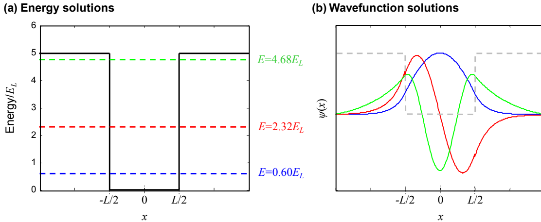
Fig. 1.23. The three bound states for electrons in a well with confining potential V_0 = 5.E_L . Note that the higher the energy, the lower the effective confining potential, and the greater the penetration into the barriers.
