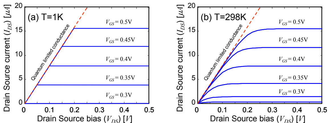
Fig. 5.25. Forward bias characteristics for a quantum wire FET at (a) T = 0K , and (b) room temperature.
