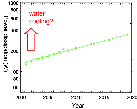
Fig. 3. Expected trends in CPU power dissipation according to the roadmap.
