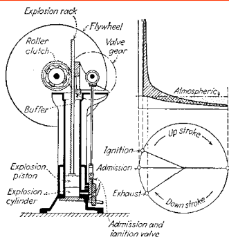
FIG. 2. Otto and Langen's free-piston engine (1806). (From "Evolution of the Internal-combustion Engine" by Edward Butler, Charles Griffin & Co., Ltd., London, 1912.)
