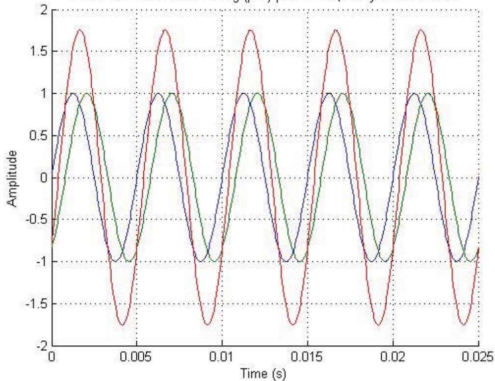
Two 200Hz sine waves: 90 deg ( \pi/2 ) phase shift; delay=1.25ms or 17^\circ
